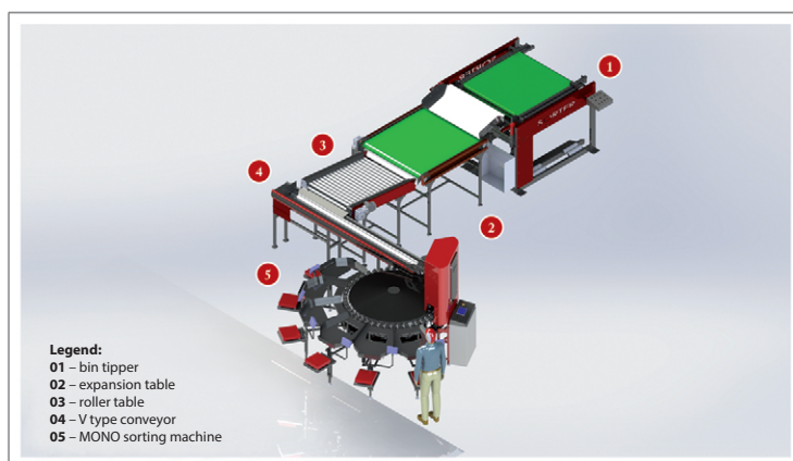
DRY UNLOADING - BIN TIPPER
