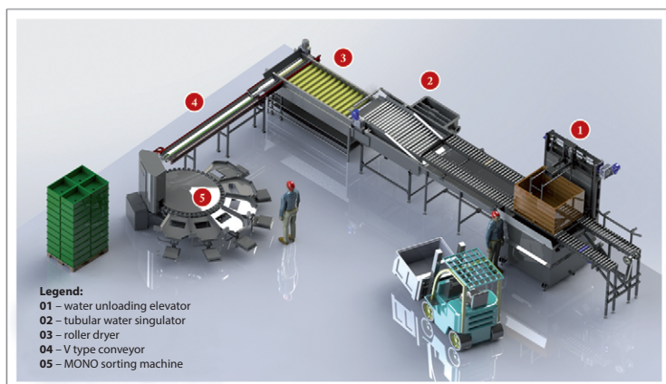
WATER UNLOADING - ELEVATOR
